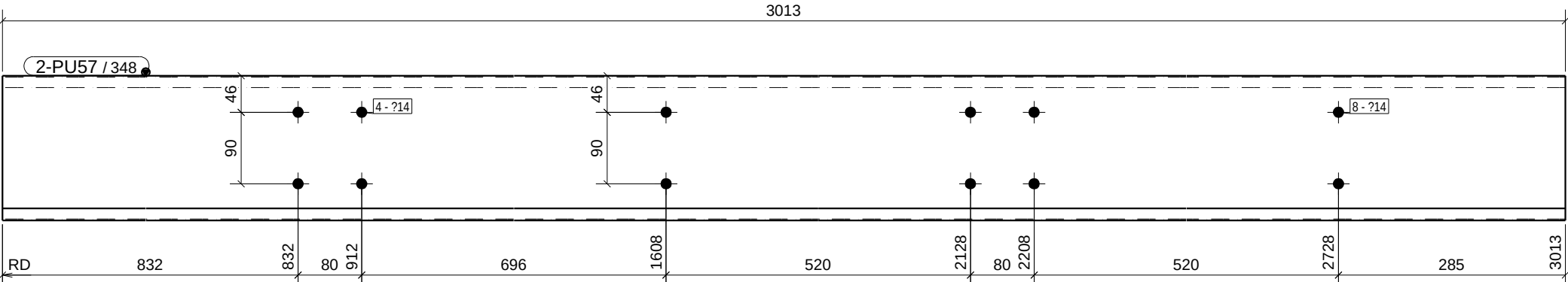
FRONT VIEW
